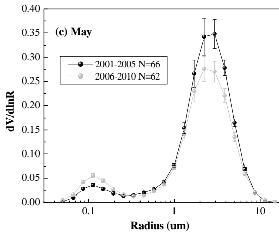
Supplementary Figure 1: Monthly mean CSDs at Kanpur AERONET station during the periods 2001-2005 and 2006-2010 for March, April and May. The number of CSD retrievals for each period is given at each graph. The vertical bars correspond to standard error from the seasonal mean.
