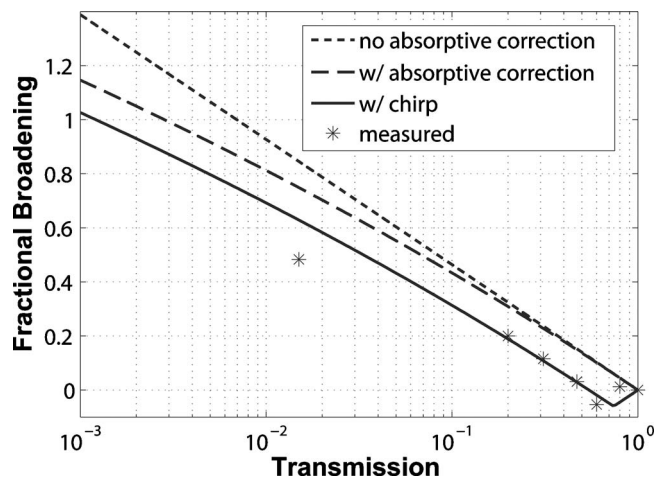
FIG. 4. Fractional pulse broadening versus natural log of transmission. Fractional broadening is defined as the fractional increase pulse duration at FWHM (a value of 0 means no broadening). Due to absorption, the actual broadening is less than that predicted by the dominant dispersive term, even though absorptive broadening is negligible.
