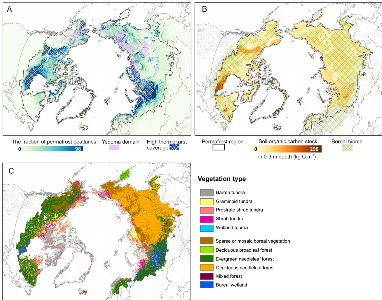
Figure 1. Maps showing (a) the permafrost peatland distribution (Hugelius et al., 2020), the distribution of Yedoma (purple; Strauss et al., 2022), landscapes with very high potential thermokarst coverage (Olefeldt et al., 2016), and (b) the distribution of the boreal biome and the soil organic carbon stocks within the permafrost region (Hugelius et al., 2014), and (c) vegetation types across the permafrost region following Virkkala et al., 2021 (note that the wetland extent on this map is likely underestimated). All maps also show the extent of the northern permafrost region as defined in the previous RECAP-2 permafrost synthesis (Hugelius et al., 2023).
