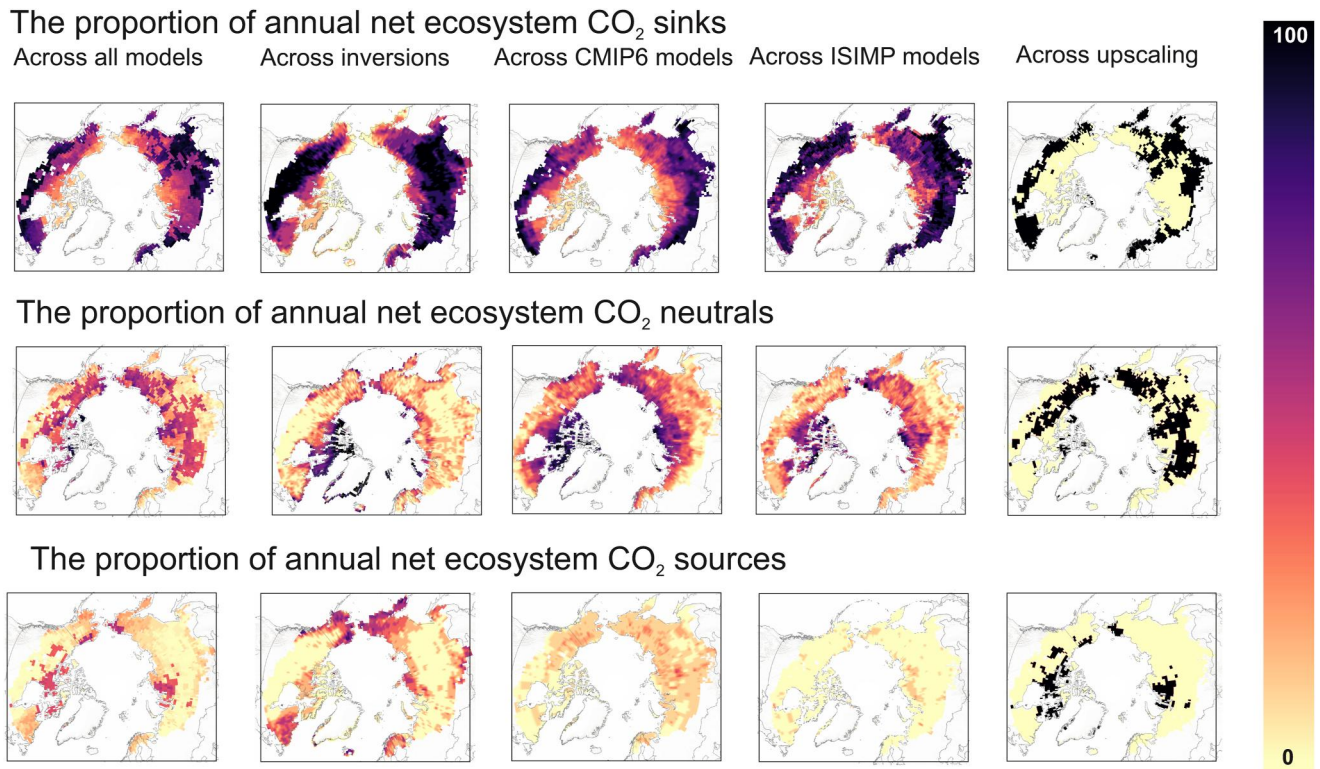
Figure 6. The proportion of models showing annual terrestrial net ecosystem CO 2 sinks (<- 10 g C m -2 yr -1 ), CO 2 neutrals (-10 - +10 g C m -2 yr -1 ), and CO 2 sources (>+ 10 g C m -2 yr -1 ). The “Across all models” map was produced so that each modeling approach (inversions, process-based, and upscaling models) received equal weight. Note that inversion estimates include lake CO 2 fluxes as well, but fossil fuel emissions, cement carbonation sink, lateral fluxes and fire emissions have been removed; and the upscaling only includes one model and agreement cannot be calculated; thus values are either 0 (not a sink/neutral/source) or 100 (is a sink/neutral/source).
