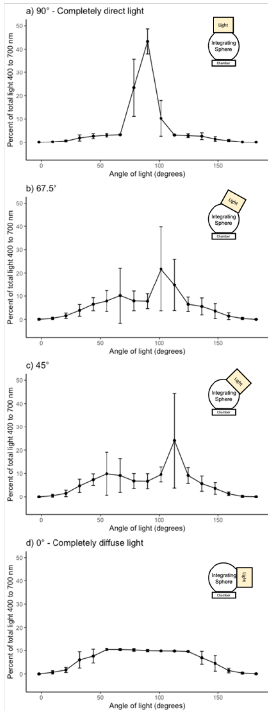
Figure 4. The percentage of light (400 to 700 nm) arriving at the leaf chamber as a function of the angular distribution of light with an integrating sphere mounted to the top of the chamber. Each panel represents the light source mounted at a different position along the track on the side including at 90° (a), 67.5° (b), 45° (c), and 0° (d). The diagram in the corner of each figure is a visual representation of the experimental setup. Data represent means and one standard deviation.
