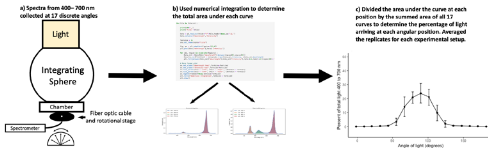
Figure 1. Workflow diagram from data collection of spectra to figures that quantify the angular distribution of light for different experimental setups of common portable plant leaf infrared gas analyzers. First (a), spectra were collected with a fiber optic connected to a rotational stage and a spectrometer. The relative intensity was collected at 17 discrete angles to capture the total light of the light source. For each spectrum (b), we used numerical integration through a programming script to calculate the total area under the curve from 400 to 700 nm. Finally (c), the total area under the curve at each angular position was divided by the summed area under the curve for all 17 spectra collected for each experimental setup. For each experimental setup, 10 to 25 replicates were conducted and averaged.
