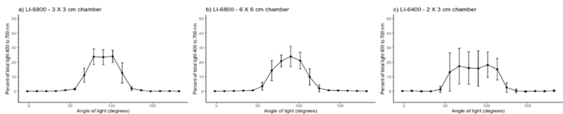
Figure 3. The percentage of light (400 to 700 nm) arriving at the leaf chamber as a function of the angular distribution of light. Data are shown for three commonly used gas exchange chambers; the LI-6800 3 x 3 cm chamber (a; “small leaf chamber”), the LI-6800 6 x 6 cm chamber (b; “large leaf chamber”) and the LI-6400XT 2 x 3 cm chamber (c). Each panel had the light source in its traditional position mounted directly above the leaf chamber. Data represent means and one standard deviation.
