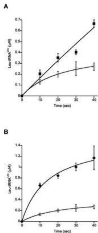
Figure 1. Effects of ProRS and TyrRS on aminoacylation by LeuRS
