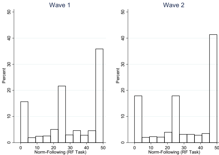
Fig. 1 Estimates of norm-following propensity
