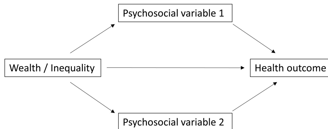
Appendix 1—figure 2. Causal diagram highlighting multiple mediation.
