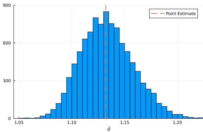
Fig. 9. Bootstrap distribution of \hat{\theta} for \bar{F} = 2.0 .
