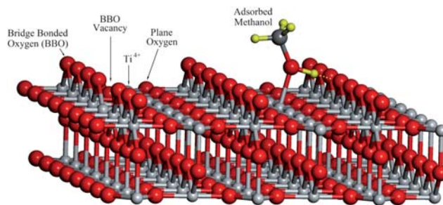
Fig. 1 The TiO 2 (110) surface model with about 4% concentration of BBO vacancy.
