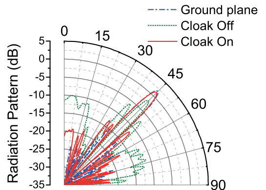
FIG. 4. (Color online) Radiation pattern for the reflected Gaussian beam from the ground plane (dash-dotted blue line), the bump without cloak (dotted green line), and from the cloaked bump (solid red line).
