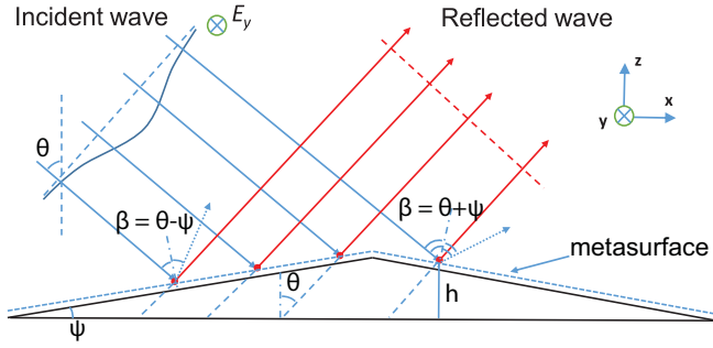
FIG. 1. (Color online) Scheme of the carpet cloak with metasurface.
