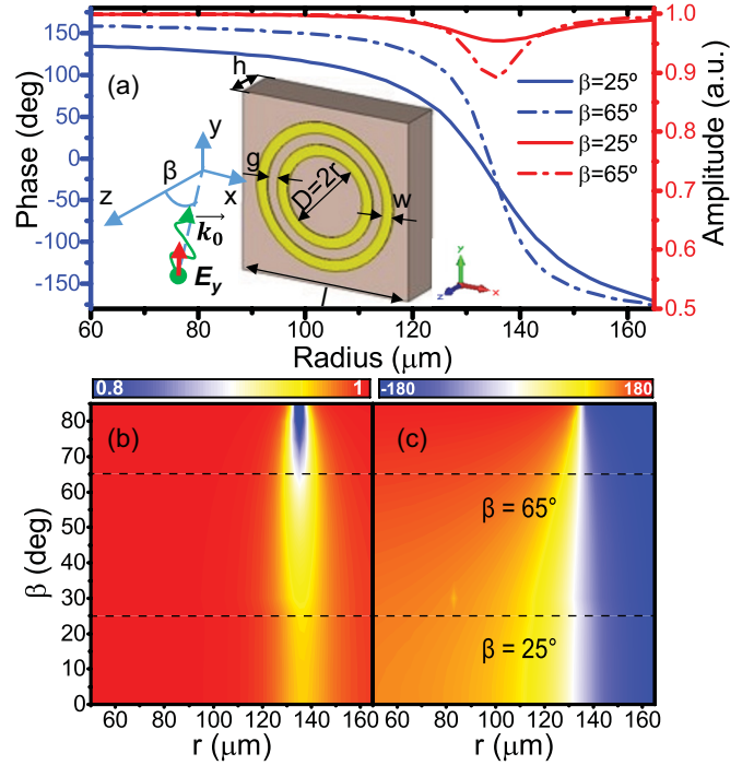
FIG. 2. (Color online) (a) Phase response of the unit cell for different angles of incidence. (Inset indicates the unit cell geometry and its corresponding parameters.) Color-map for the amplitude (b) and phase (c) of the reflection coefficient as a function of the incidence angle and radius of the inner ring.
