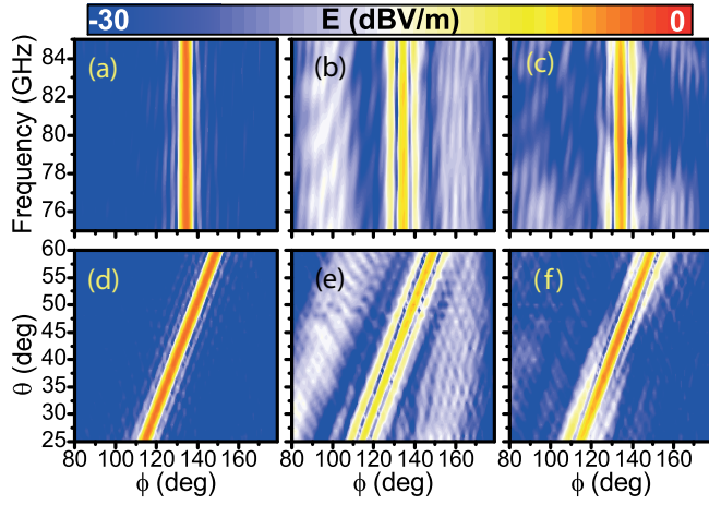
FIG. 5. (Color online) Amplitude of the far-field component of the electric field as a function of azimuth angle \phi and frequency (a)–(c) and as a function of the incidence angle \theta and azimuth angle \phi (d)–(f). Left column refers to the beam reflected from the ground plane, center from the bare bump, and right column from the bump covered with the cloak.
