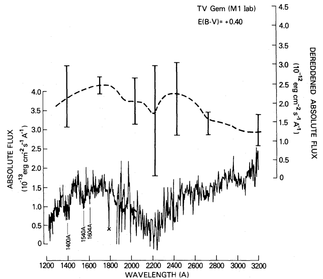
FIG. 1.—TV Gem absolute flux plotted against wavelength from observations obtained 1979 November 25 where both short and long wavelength spectral images are shown together ( \sim 6 \text{ \AA} spectral resolution). Data were obtained with the 10'' \times 20'' entrance slit of IUE . A number of broad absorption features are noticeable in the 1400 \text{\AA} –1600 \text{\AA} range. The data corrected for interstellar absorption ( dashed curve ) is shown for an E(B-V) = +0.40 . Error bars indicate uncertainty in the measured continuum flux level obtained using 10 minute exposures; \times indicates a reseau mark.
