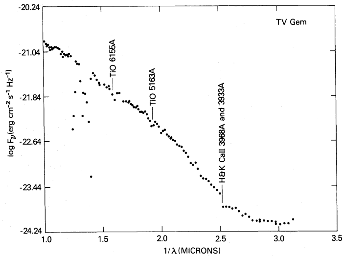
FIG. 2.— Multichannel scanner spectrum of TV Gem obtained by J. B. Oke on 1980 January 25 on the 200 inch telescope. The rapidly decreasing continuum with decreasing wavelength is expected for an M1 supergiant. TiO bands typical of cool stars are present and their strength is consistent with an M1 spectral designation. Below 3600 Å the continuum is dominated by the hot companion. The measured flux from these data at 3200 Å agrees within a factor 2 with IUE calibrated flux estimates.
