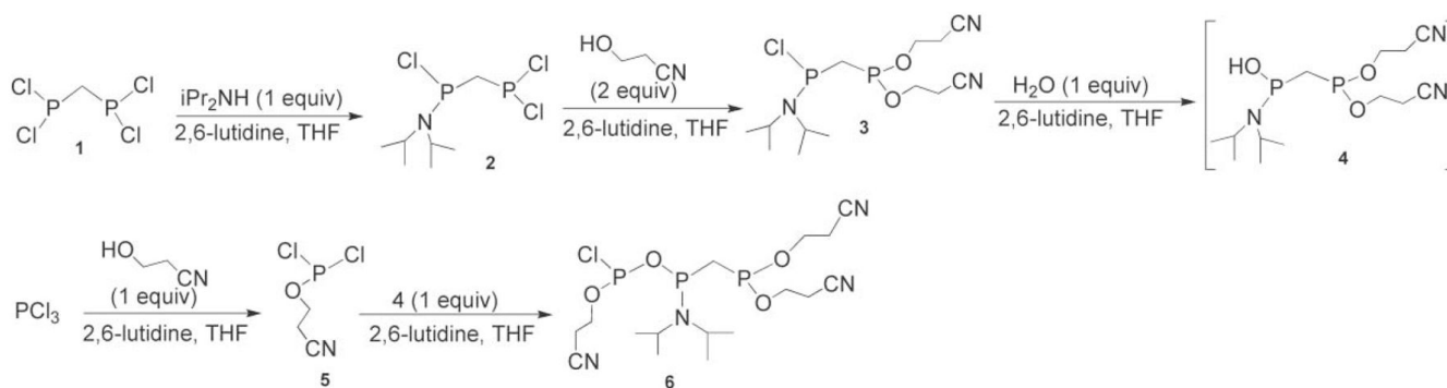
Scheme 1. Synthesis of \alpha,\beta -methylene- \beta -triphosphitylating reagent 6 .
