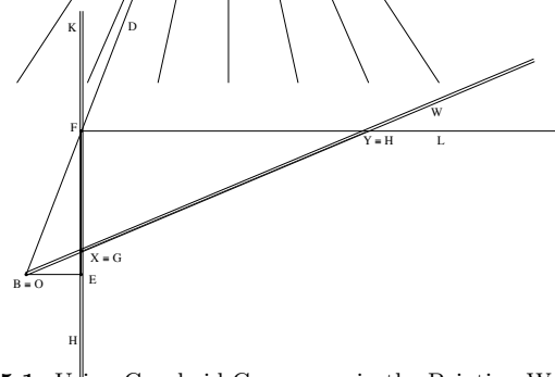
Figure 5.1: Using Conchoid Compasses in the Pointing Way
