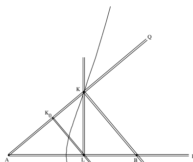
Figure 8.3: A Modification of the Instrument Suggested by Clavius's Solution of the Two Mean Proportionals Problem
