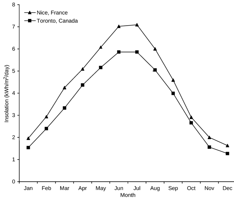
Fig. 2. Monthly solar insolation values for cities at the same latitude. Locations at the same latitude may have very different solar insolation due to local conditions. The latitude of Nice, France, is 43.70 degrees N, with a maximum monthly increase in solar insolation of 1.31 kWh/m 2 /day between February and March. The latitude of Toronto, Canada is 43.67 degrees N, with a maximum monthly increase in solar insolation of 1.04 kWh/m 2 /day between March and April.
