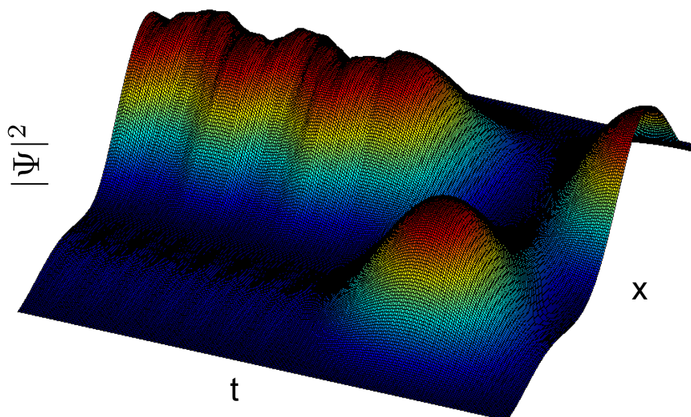
Figure 5. The initial probability amplitudes for |\psi(x,0)|^2 appear on the right of the figure, and time evolves to the left. After one revival period, when the zero has reappeared at x_0 = \frac{3}{8}L , an infinite barrier is raised there, and the state evolves for the same period in the new potential.
