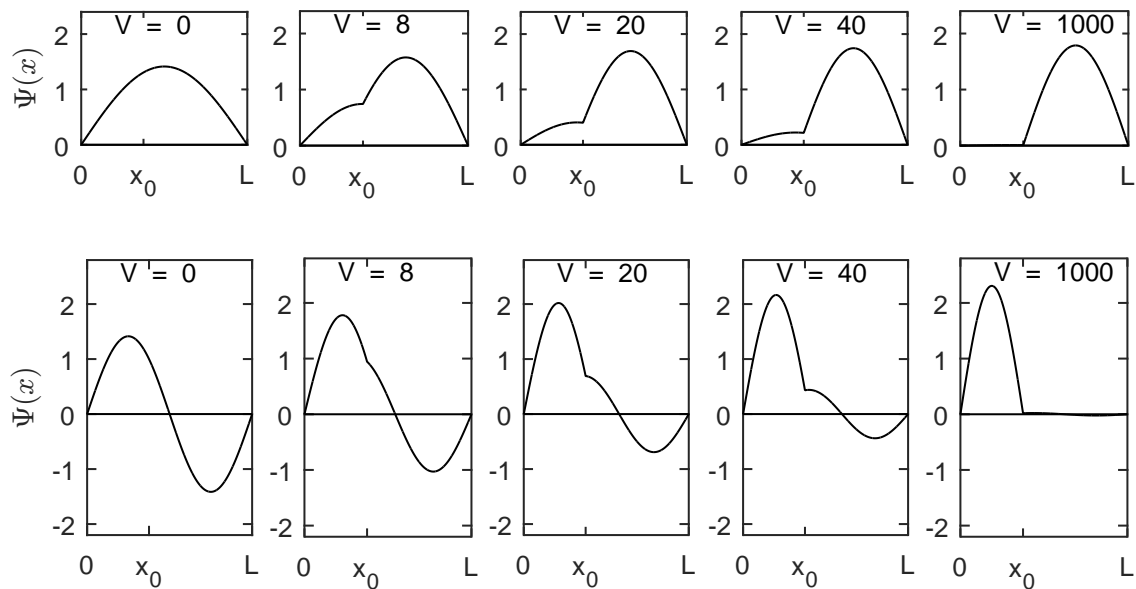
Figure 3. The ground state (top) and first excited state (bottom) of the infinite square well with a delta-function potential of magnitude V located at x_0 = \frac{3}{8}L . Clearly, as the barrier magnitude increases each eigenstate becomes confined on one side of the barrier or the other, becoming eigenstates of the individual wells.
