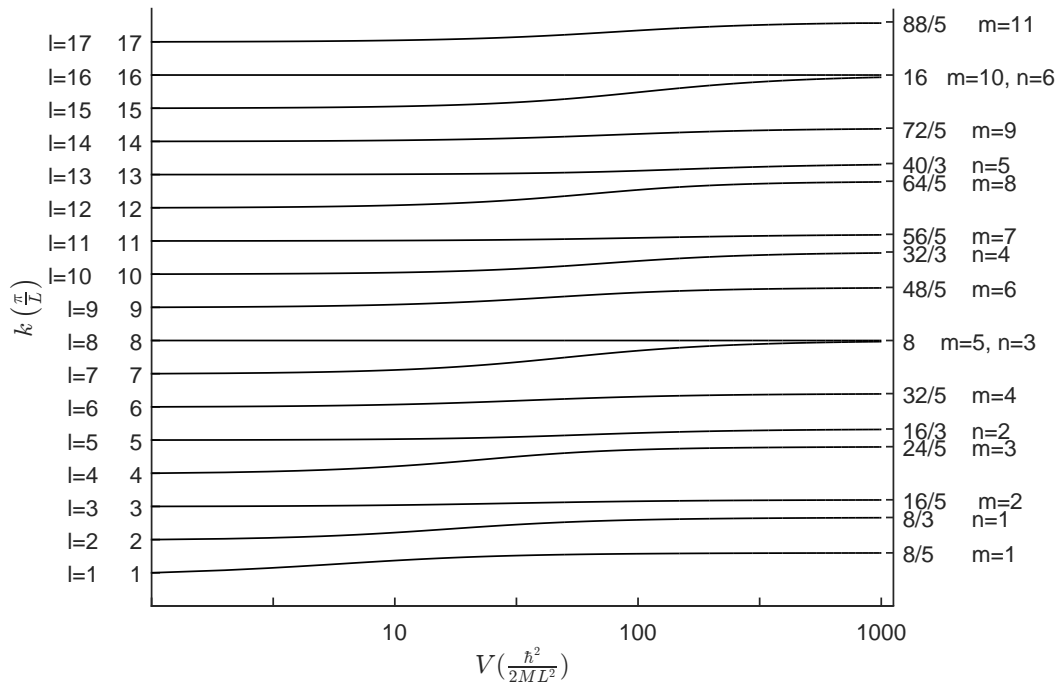
Figure 2. Spectrum of the infinite square well with a delta-function potential of magnitude V located at x_0 = \frac{3}{8}L . The levels are shown in terms of the wave number k = \sqrt{2ME} and a logarithmic scale for V (which has units of [\hbar^2/2ML^2] ).
