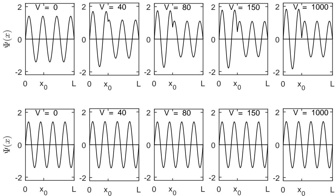
Figure 4. The seventh (top) and eighth (bottom) excited state of the infinite square well with a delta-function potential of magnitude V located at x_0 = \frac{3}{8}L . These eigenstates become degenerate and clearly fail to become confined on one side of the barrier or the other as the barrier magnitude increases, and thus they do not become eigenstates of the individual wells. Instead, the eigenstates of the individual wells are orthogonal superpositions of these two eigenstates of the original well, as shown in Equations (18) and (19).
