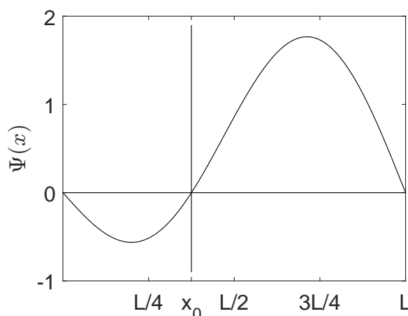
Figure 1. Plot of \psi(x) with x_0 = \frac{3}{8}L where a sudden barrier can divide the well.
