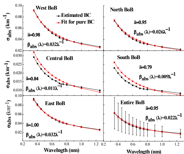
Fig. 16. Wavelength dependence of the absorption coefficient for estimated BC (OPAC) and that for pure BC assuming an absorption wavelength exponent \tilde{a} = 1 .
