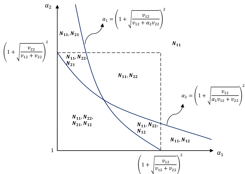
Figure 2: The Equilibria Conditions.
