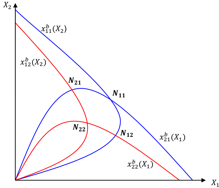
Figure 1: The Equilibria.
